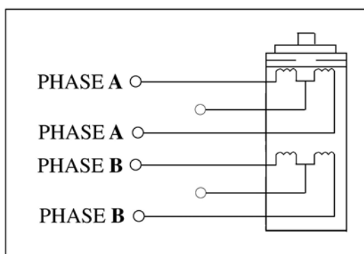
Figure 8: 6 Lead Full Coil (Higher Torque) Motor
