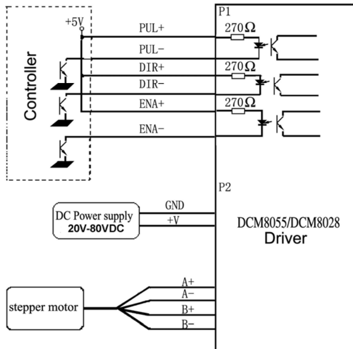
Figure 10: Driver connection in a stepping system
