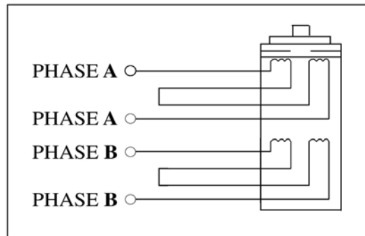
Figure 5: 8 Lead Motor Series Connections
