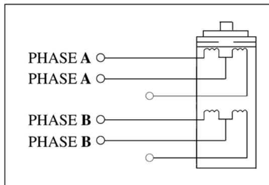
Figure 7: 6 Lead Half Coil (Higher Speed) Motor Connections
