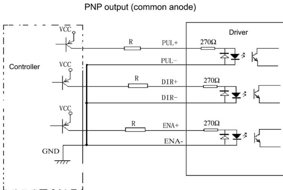
Figure 3: Signal Interface
