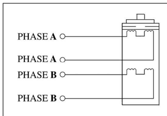
Figure 9: 4 Lead Motor Connections
