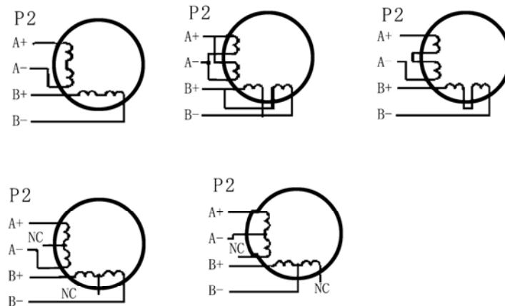
Figure 4: Driver Connection to Step Motor
