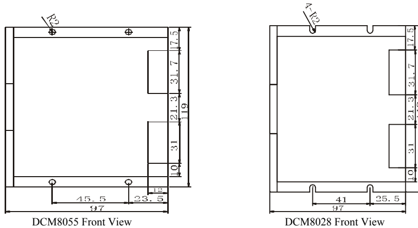
Figure 1: Mechanical Dimensions
